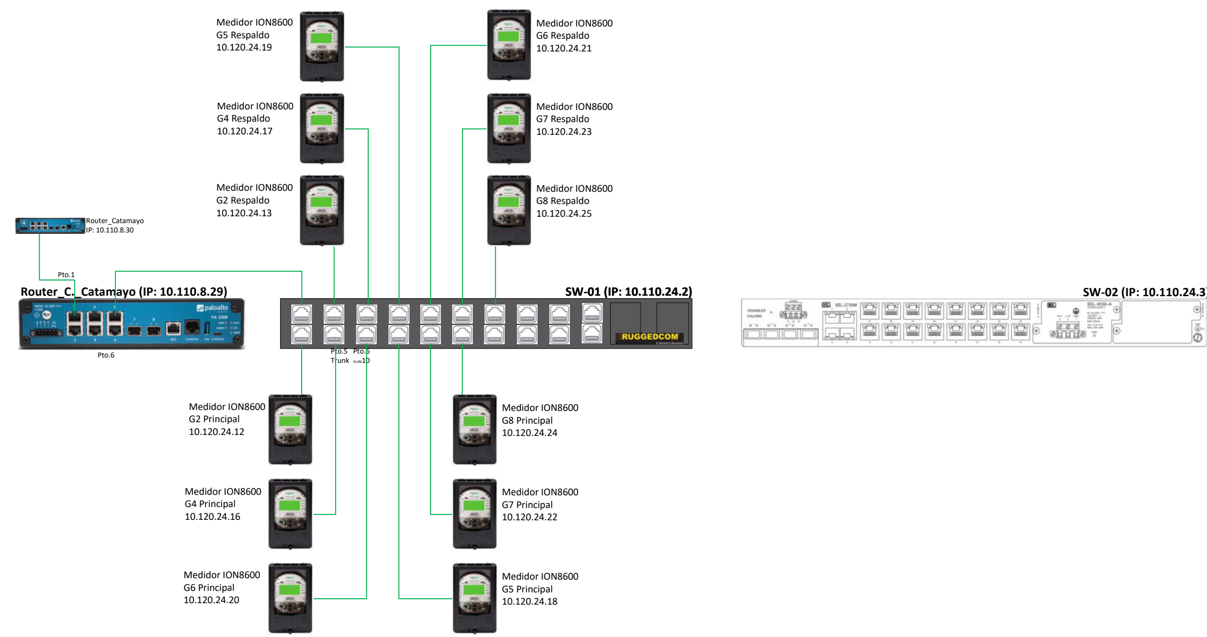
Diagrama Central Catamayo
